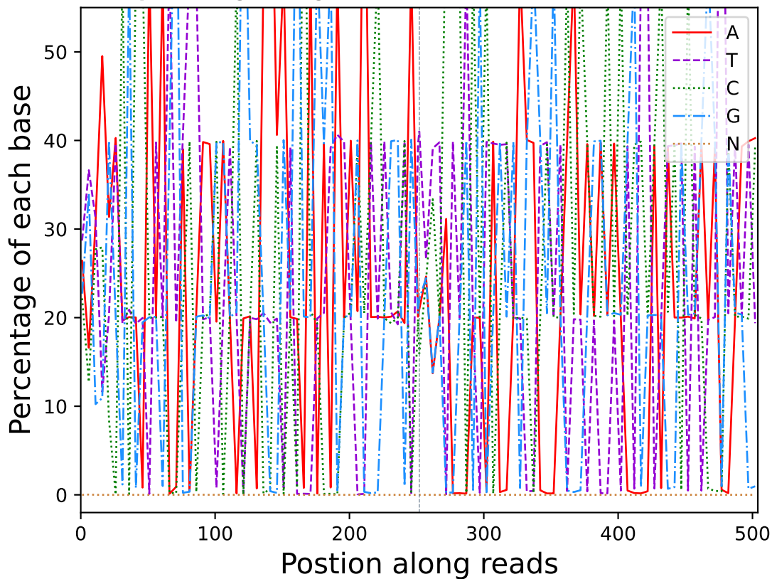
Base percentage along reads (R10421)
